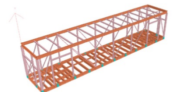
Figure 4: Structural model of local control room for seismic and wind analysis
