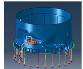
Figure 2: Potential buckling failure of LN tank failure base from finite element analysis
